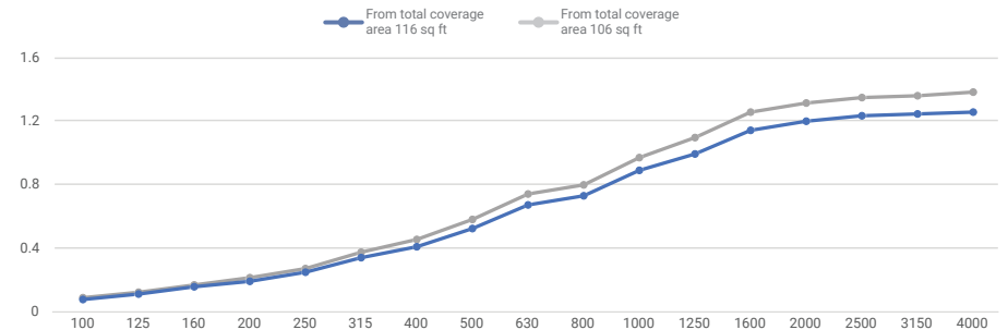
Beams NRC Comparison for 94.5"x84"x5.9" OC-24" [2400x2133x150mm OC-609mm]
