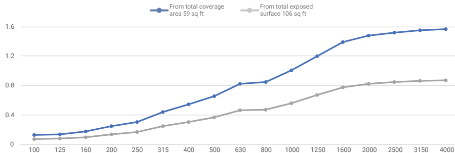
Beams NRC Comparison for 94.5"x84"x5.9" OC-12" [2400x2133x150mm OC-305mm]
